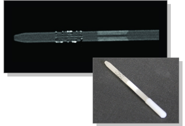
Example for a Stent-phantom based on CTiodine® and providing a stenosis (calcification).
